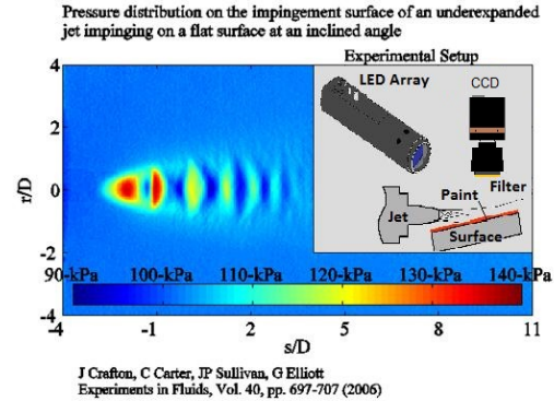
Example of pressure measurements accomplished using UniFIB™ PSP
