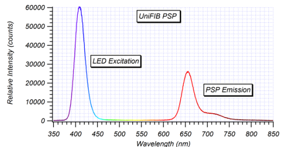
Emission spectra of UniFIB™ PSP. Paint excited using LM2X-DM-400 LED.
