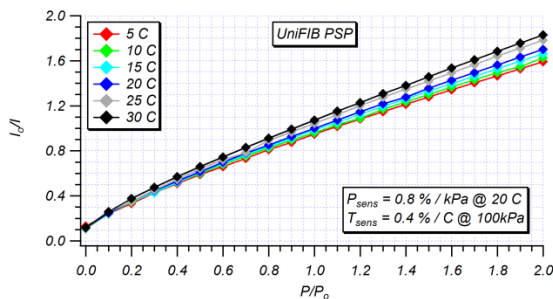
Calibration of UniFIB™ PSP
